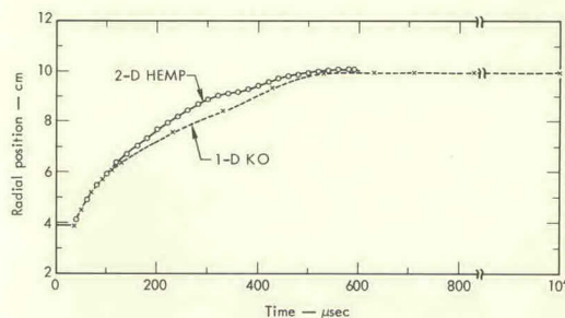
FIG. 4. Radial position of He-steel-wall boundary vs time (1-D KO code results and 2-D HEMP code results taken from axial midpoint of HE).
