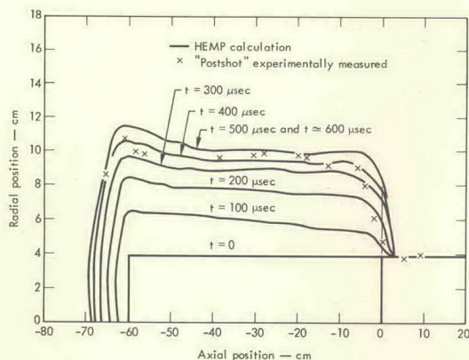
FIG. 3. Position of He-steel-wall boundary from HEMP plotted at 100- \mu\text{sec} intervals. "Postshot" measured values are also shown.
